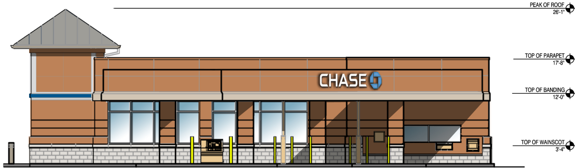
EAST ELEVATION
